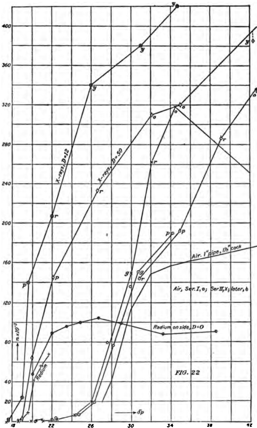
FIG. 22—Efficient nucleation ( n ) found in dust-free air energized or not by radium or the X-rays, as stated, from different distances ( D ), at different exhausts ( \delta p ). Fog chamber with pipes 1 1/4-inch bore, 2 feet long. Table 13.
